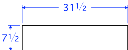
PV 7-1/2"W x 31-1/2"L x 1.5"H
