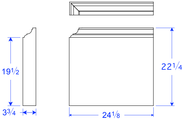
BM 26-19.5 LR 22 1/4"H x 24 1/8"L x 3 3/4"T
