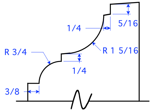
BM 26 Profile Note: BM 26-20 is 3 1/2" Thick Not To Scale
