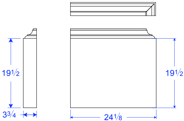
BM 26-19.5 RR 22 1/4"H x 24 1/8"L x 3 3/4"T
