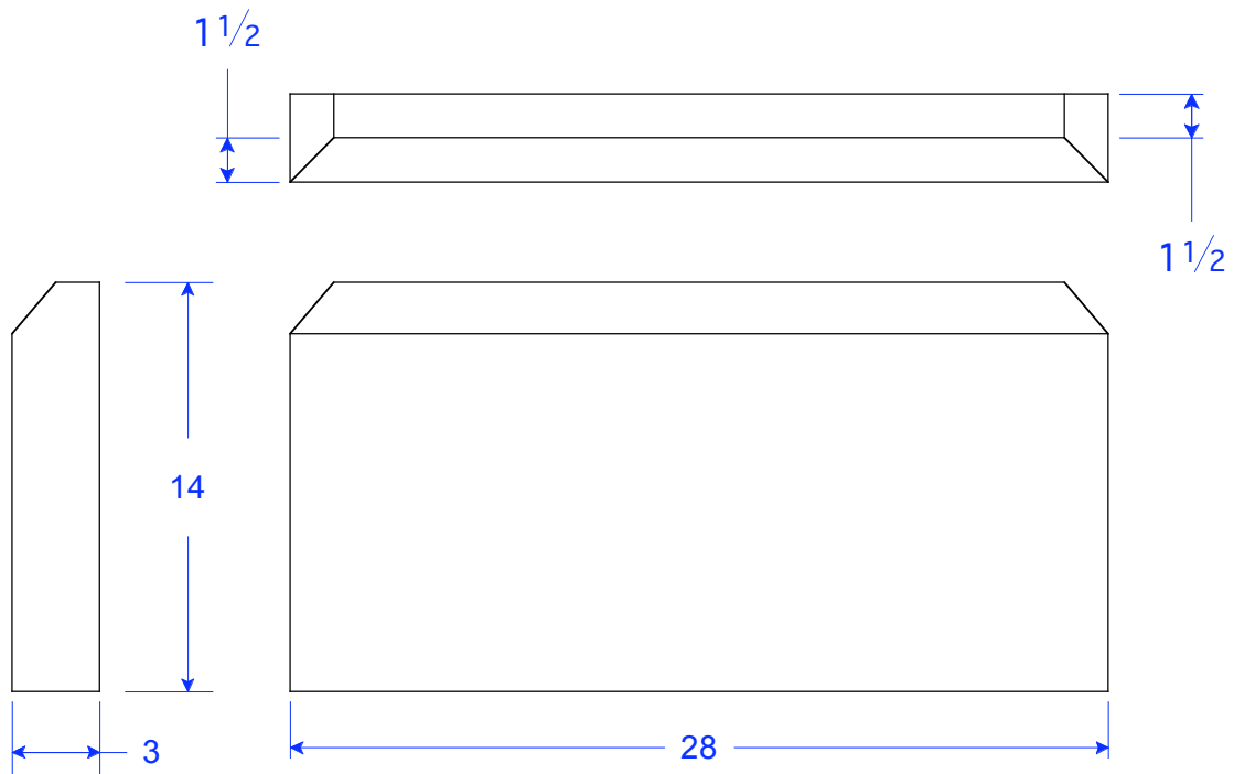
BM 34-3x14 DR 14"H x 28"L x 3"T
