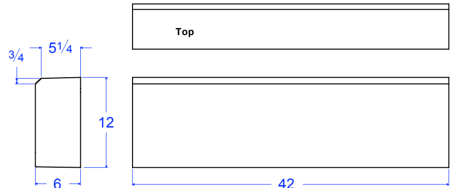
BM 34-6x12x42 6"W x 42L x 12"H
