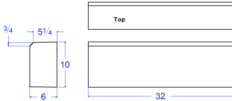
BM 34-6x10x32 6"W x 32L x 10"H
