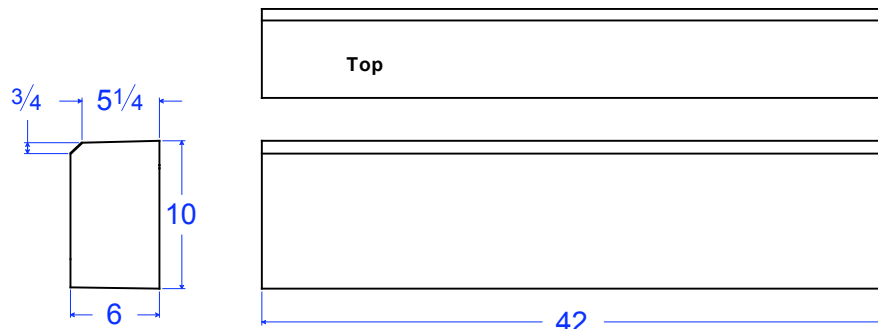
BM 34-6x10x42 6"W x 42L x 10"H
