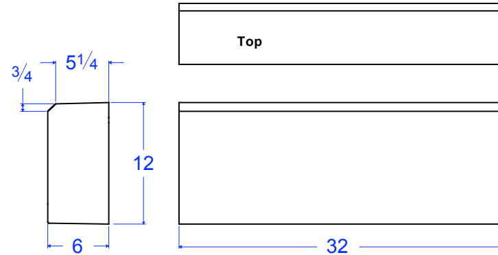
BM 34-6x12x42 6"W x 42L x 12"H
