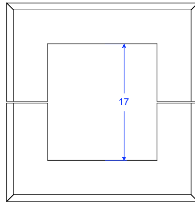
CLT 24 & 25 BE Column Base Extension 14 3/8W x 28 Lx 4 1/2H
