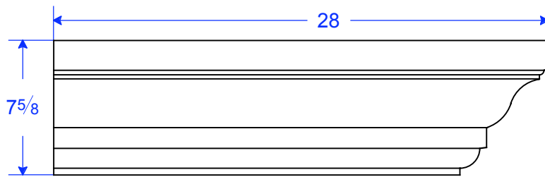
CM 27-2 RR 7 5/8"H x 28"L x 6 1/2"T
