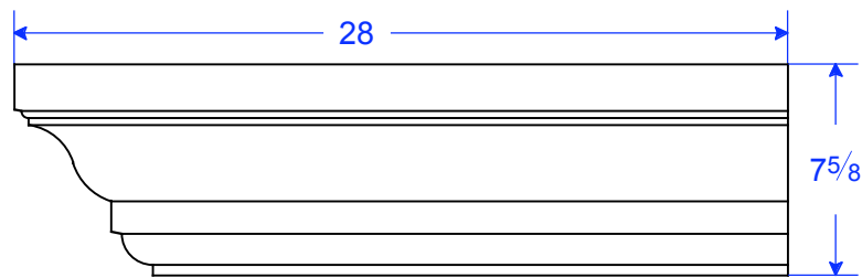
CM 27-2 LR 7 5/8"H x 28"L x 6 1/2"T
