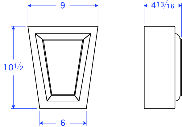
KS 18-10.5 9"W x 10 1/2"H x 4 13/16"T
