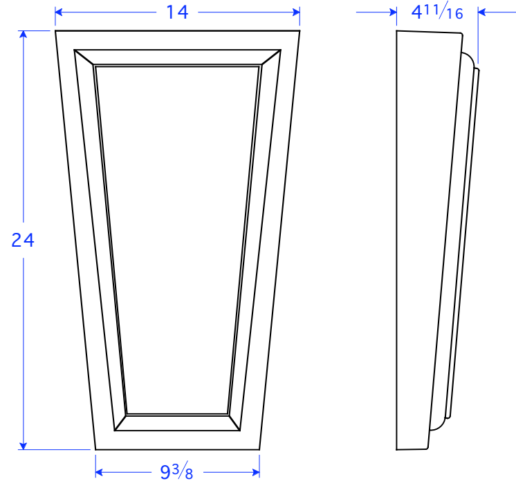
KS 18-24 24"W x 14"H x 4 11/16"T
