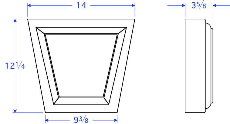
KS 18-12 12 1/4"W x 14"H x 3 5/8"T
