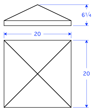
PC 13-20 P6.25 20"W x 20"L x 6 1/4"H
