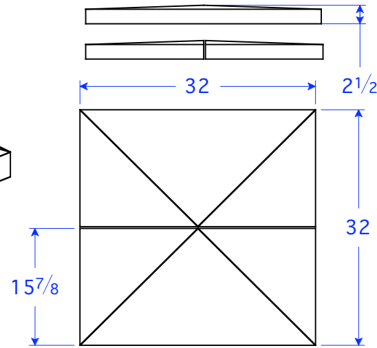
PC 13-16 P2.5* 15 7/8W x 32L x 2.5H * Two Pieces Needed To Make A Pier Cap 32 x 32 x 2.5
