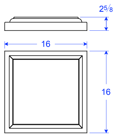
PC 18-16 F 16"W x 16"L x 2 5/8"H
