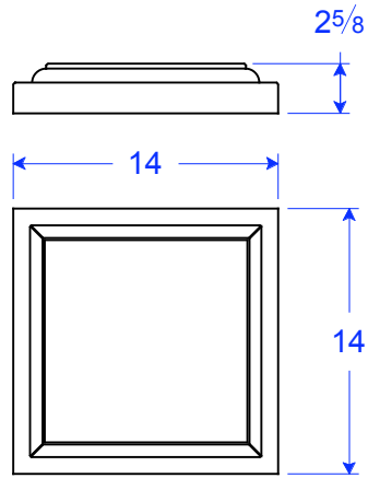
PC 18-14 F 14"W x 14"L x 2 5/8"H
