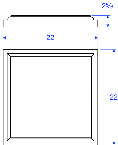
PC 18-22 F 22"W x 22"L x 2 5/8"H
