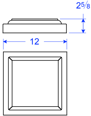
PC 18-12 F 12"W x 12"L x 2 5/8"H
