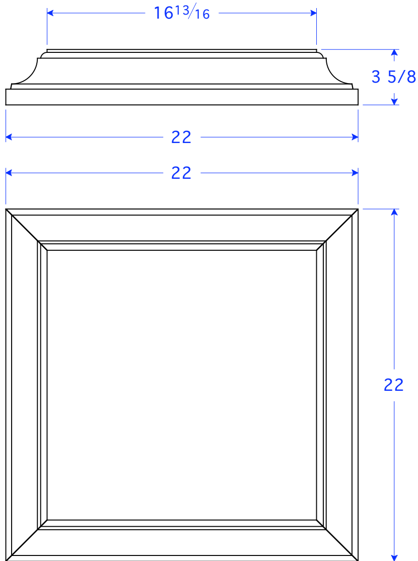
PC 26 F 22"W x 22"W x 3 5/8" (Flat top)
