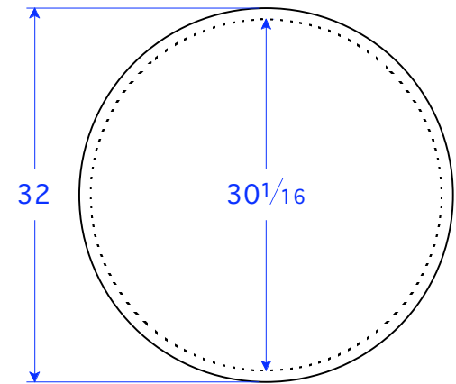
PC 36-34.5 RD 32"OD x 3 1/4" H
