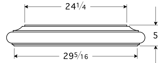
PC 56-5x33 F 29 5/16"SQ x 3"H
