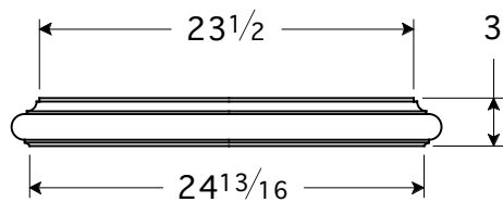
PC 56-3x27 F 24 13/16"SQ x 3"H
