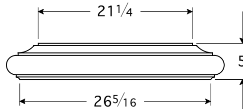
PC 56-5x30 F 26 5/16"SQ x 3"H
