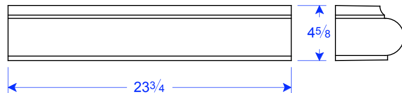
PL 01-12 x 4.5 Extension 23 3/4"W x 4 5/8"H x 5 3/4"D
