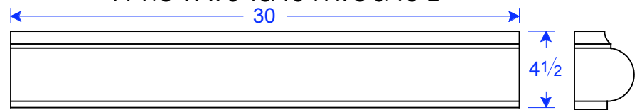
Extension for PL 01-7.56 x 4.5 30"W x 4 1/2"H x 3 9/16"D
