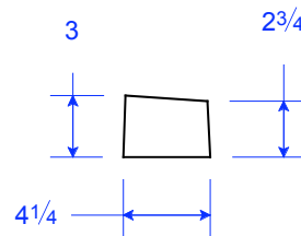
SM 02-04.25x3x32 4 1/4"W x 32"L x 3"H
