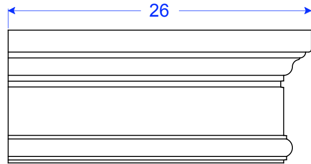
TM 12-4 RR 11 3/8"H x 26"L x 5 5/8"T
