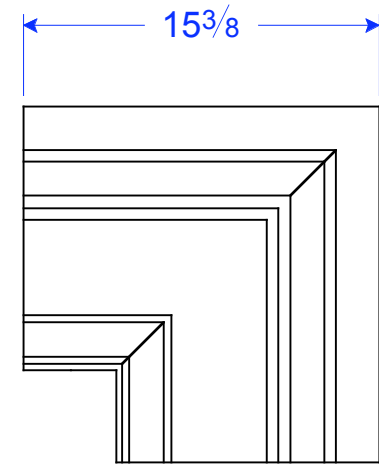
TM 12-4 CF 15 3/8"H x 15 3/8"L x 5 5/8"T
