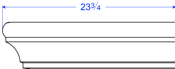
TM 19 LR 6 7/16"H x 23 3/4"L x 3 13/16"T
