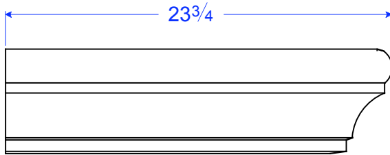
TM 19 RR 6 7/16"H x 23 3/4"L x 3 13/16"T
