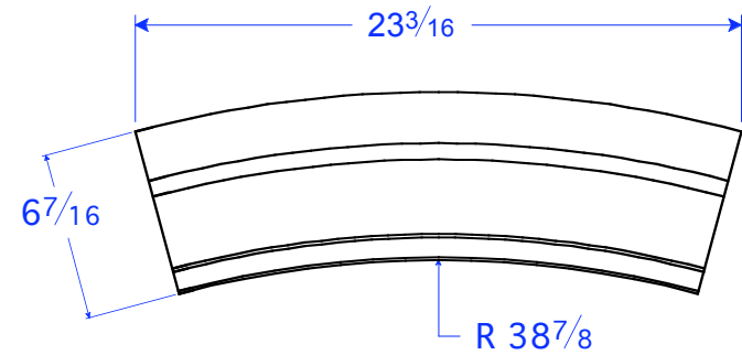
TM 19 STR R 38 7/8" 6 7/16"H X 23 3/16"L X 3 13/16"T
