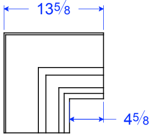
TM 21 CF 13 5/8"H x 13 5/8"L x 4 1/2"T
