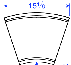
TM 24-12 STR R 12 1/2" 11 1/2"H x 15 1/8"L x 1 7/16"T
