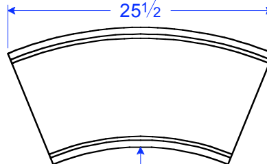
TM 24-12 STR R 22 1/8" 11 1/2"H x 25 1/2"L x 1 7/16"T
