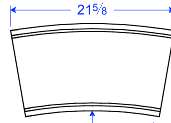
TM 24-12 STR R 51 9/16" 11 1/2"H x 21 5/8"L x 1 7/16"T
