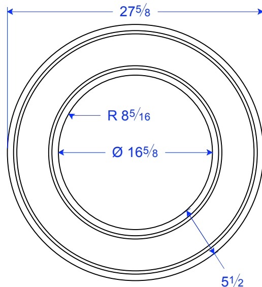
TM 24-5 QT RD 16 5/8"ID x 27 5/8"L x 1 7/16"T
