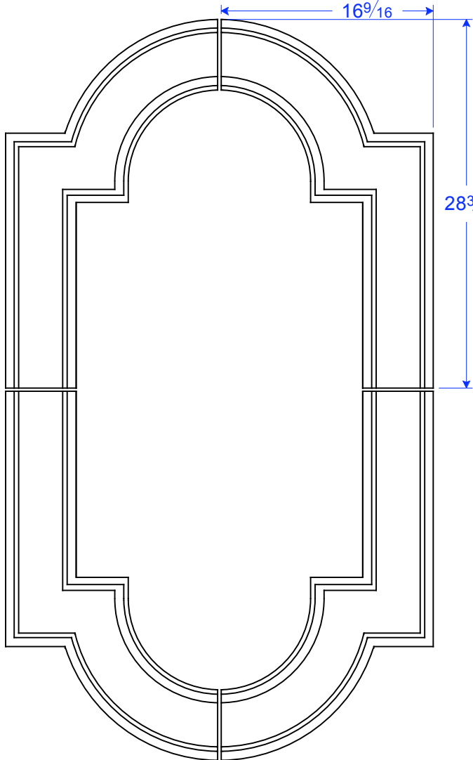
TM 24-5 QT 4P 57 3/4"H x 33 3/8"L x 1 7/16"T
