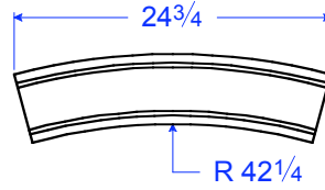
TM 24-5 STR R 42 1/4" 5 1/2"H x 24 3/4"L x 1 7/16"T
