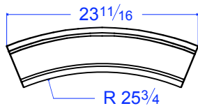
TM 24-5 STR R 25 3/4" 5 1/2"H x 23 11/16"L x 1 7/16"T
