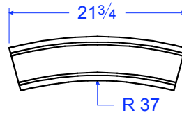
TM 24-5 STR R 37" 5 1/2"H x 21 3/4"L x 1 7/16"T
