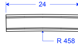
TM 24-5 STR R 458" 5 1/2"H x 24"L x 1 7/16"T
