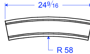
TM 24-5 STR R 58" 5 1/2"H x 24 9/16"L x 1 7/16"T
