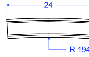
TM 24-5 STR R 194" 5 1/2"H x 24"L x 1 7/16"T
