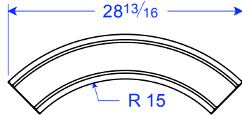
TM 24-5 STR R 15" 5 1/2"H x 28 13/16"L x 1 7/16"T
