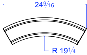
TM 24-5 STR R 19 1/4" 5 1/2"H x 24 9/16"L x 1 7/16"T
