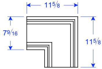
TM 24-8 CF 11 5/8"H x 11 5/8"L x 1 7/16"T
