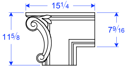
TM 24-8 CF Roco 11 5/8"H x 15 1/4"L x 1 7/16"T
