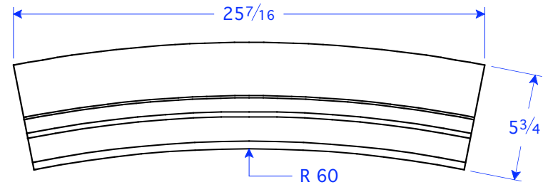
TM 26-3 STR R60 " 5 3/4"H x 25 7/16"L x 3 3/4"T
