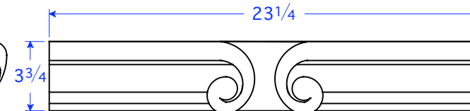
TM 26-6M STR Cor 6"W x 23 3/4"L x 3 3/4"H
