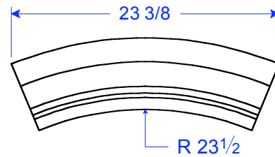
TM 30 STR R23.5 6"H x 23 3/8"L x 2 1/8"T
