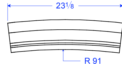
TM 30 STR R91 6"H x 23 1/8"L x 2 1/8"T
