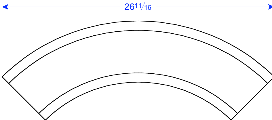
TM 32 STR R 13" 6"W x 26\frac{11}{16} "L x 3"T
